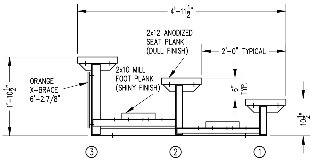
SECTION AA 3/4" = 1'-0"
