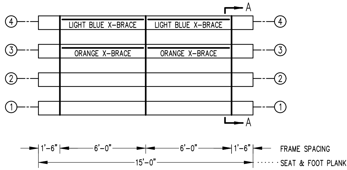
SEAT & FRAMING PLAN 1/4" = 1'-0" 40 NET SEATS @ 18" PER SEAT
