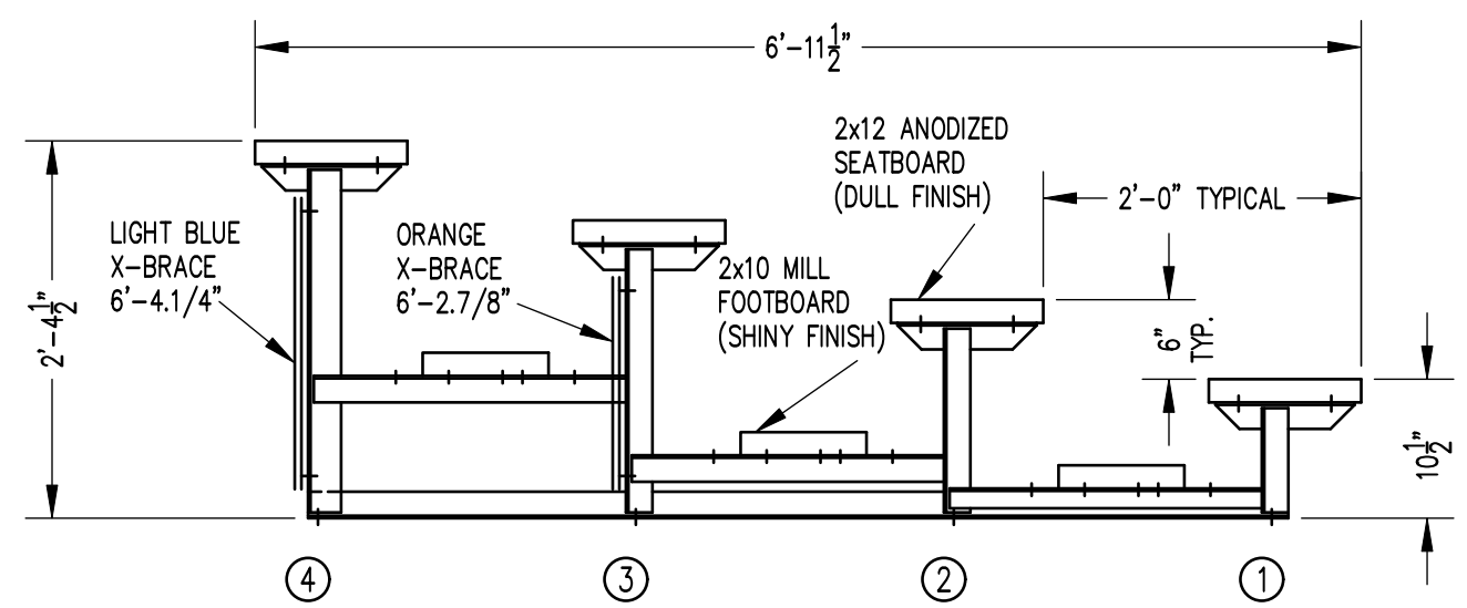
SECTION AA 3/4" = 1'-0"
