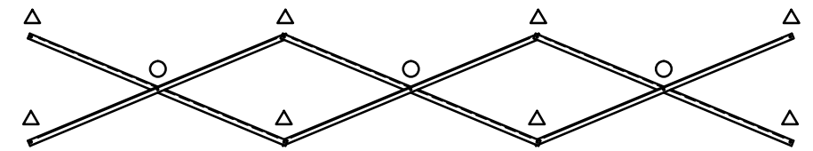
X-BRACE DETAIL N.T.S. ○ 7/16" X 1" GALV. MACH. BOLT △ 7/16" X 3" GALV. MACH. BOLT
