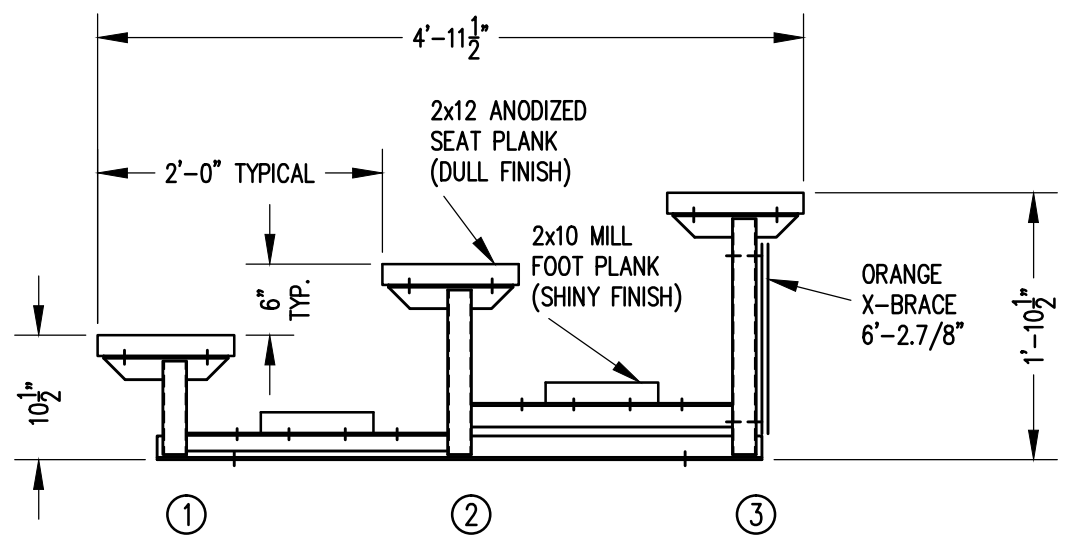
SECTION AA 3/4" = 1'-0"
