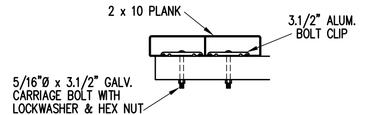
BOLT CLIP DETAIL
