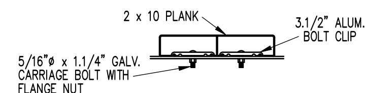
BOLT CLIP DETAIL 1.1/2" = 1'-0"
